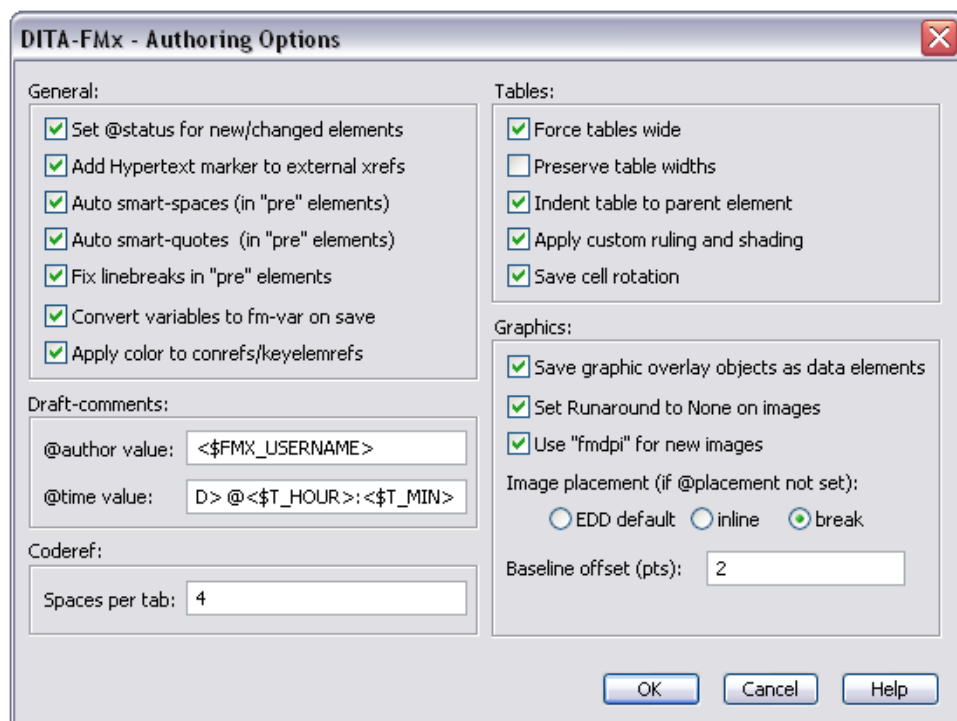
Figure 3-20: DITA-FMx Authoring Options dialog box
