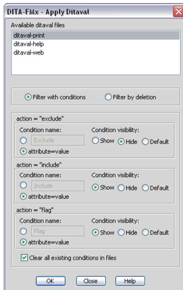
Figure 3-4: DITA-FMx Apply Conditions dialog box
